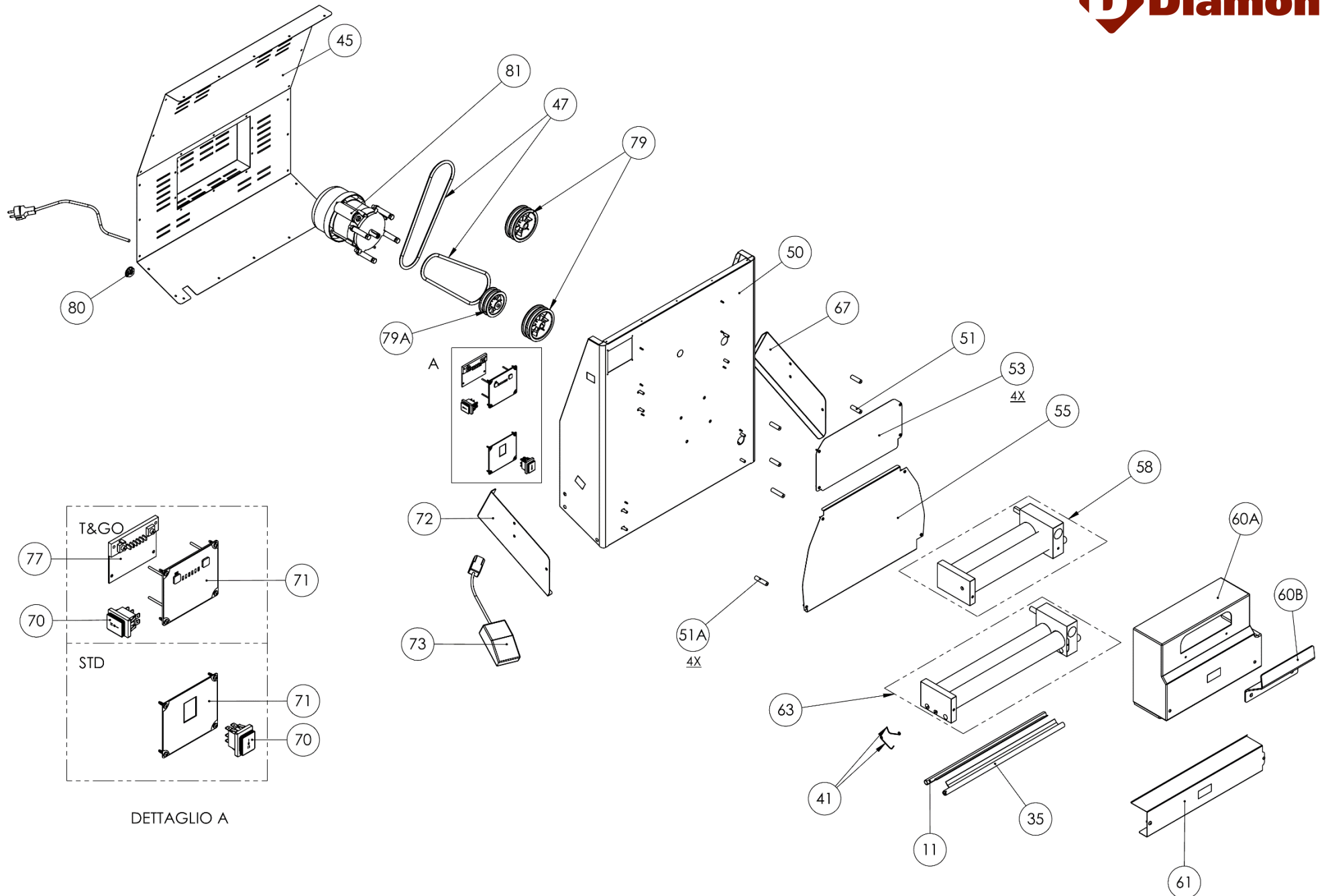
EXPLODED VIEW L42/XR
