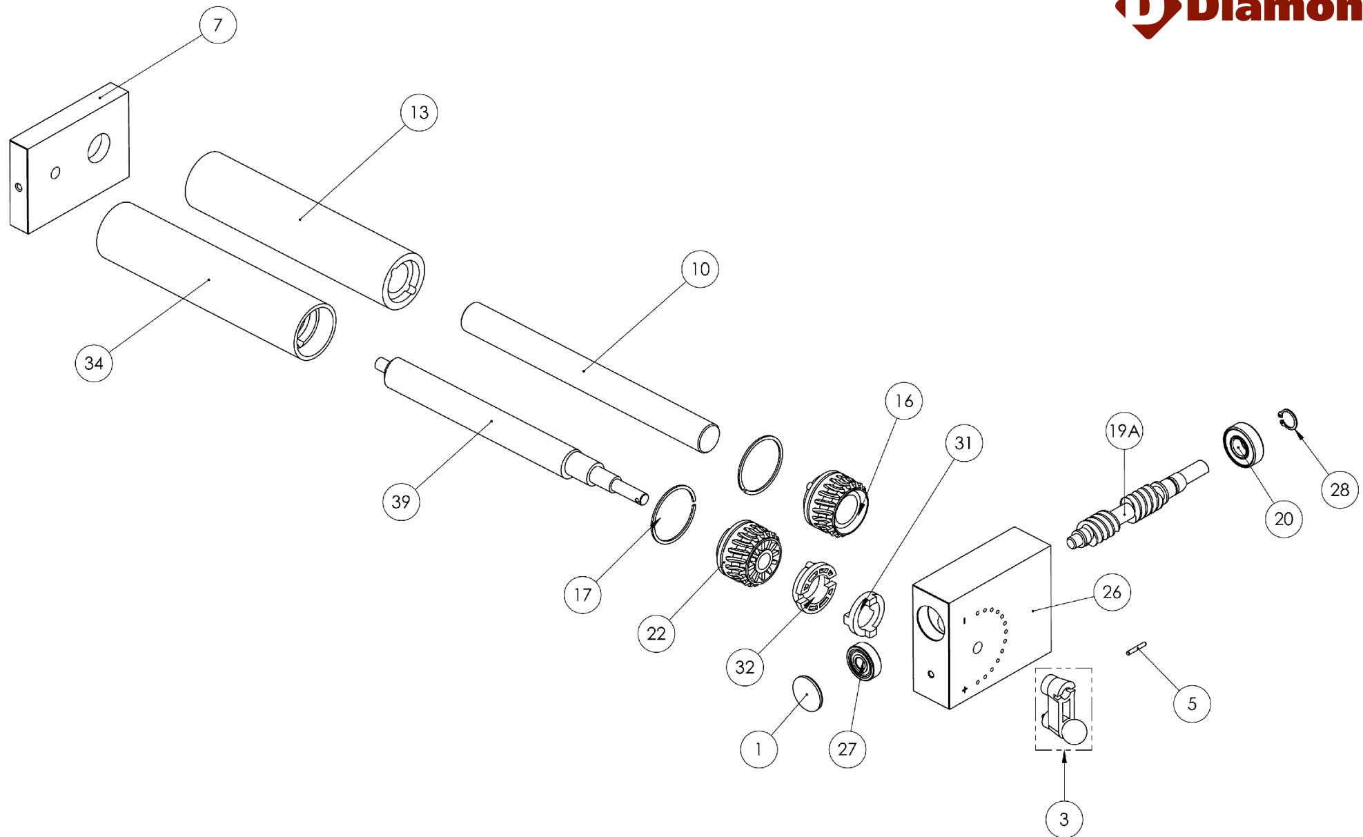
UPPER ROLLER GROUP R32/XP R42/XM L42/XR
