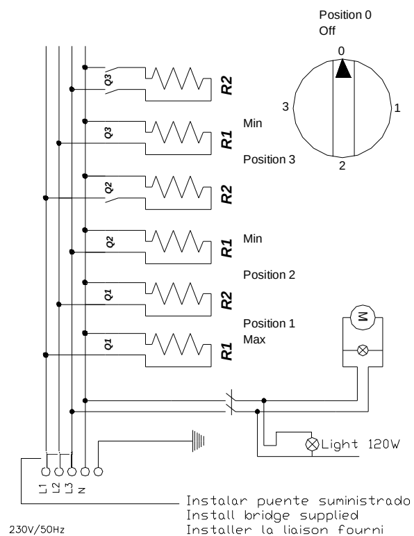
Electric diagram REV Singlephase
