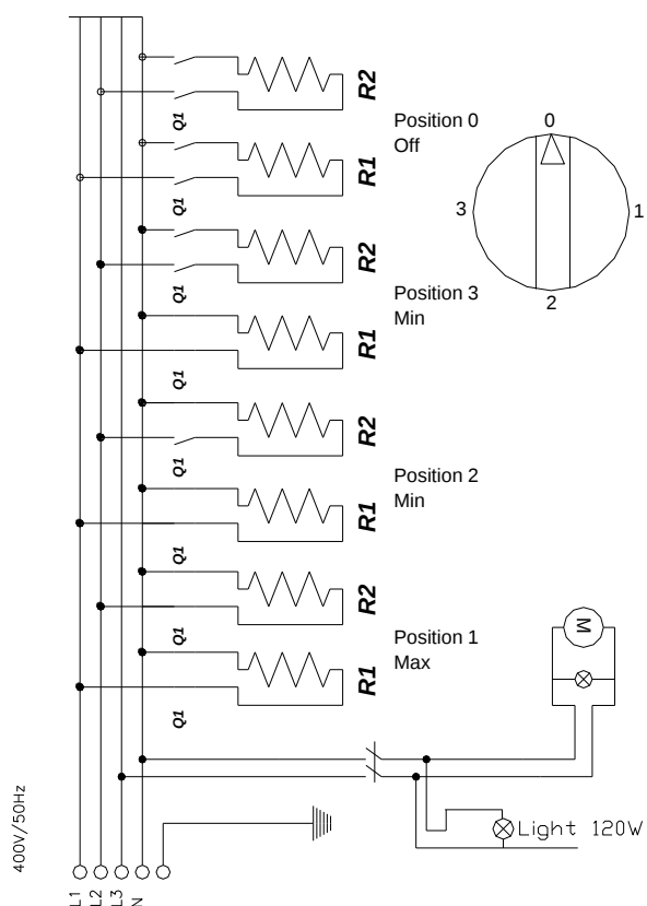
Electric diagram REV
