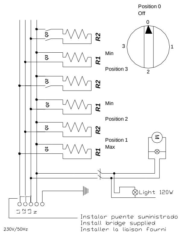
Electric diagram REV Singlephase
