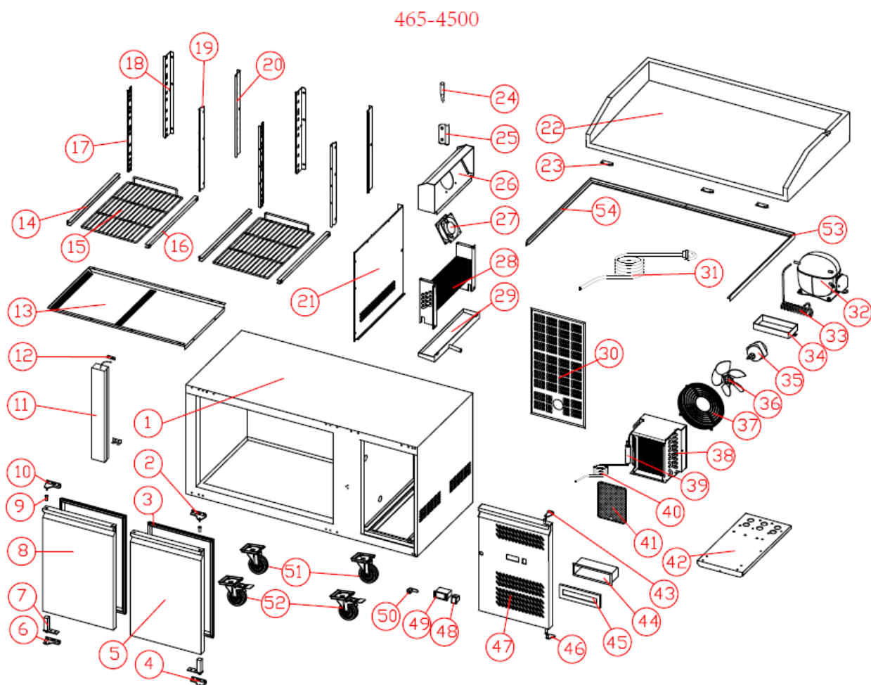
EXPLODED VIEW
