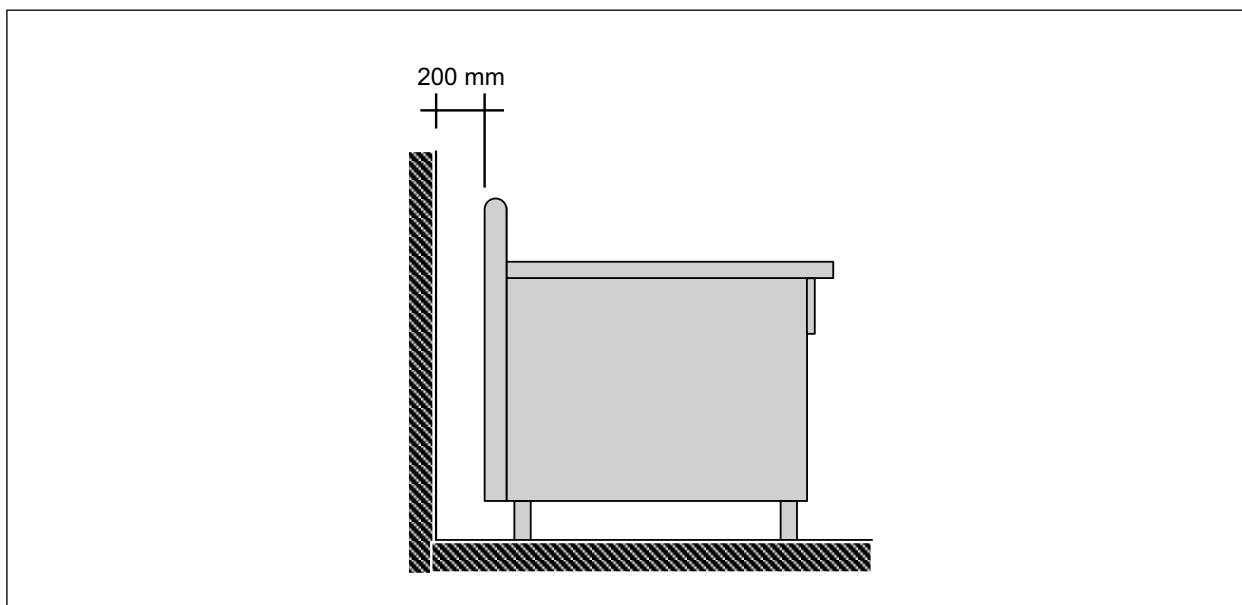
Fig. 21 Minimum distance from flammable walls
