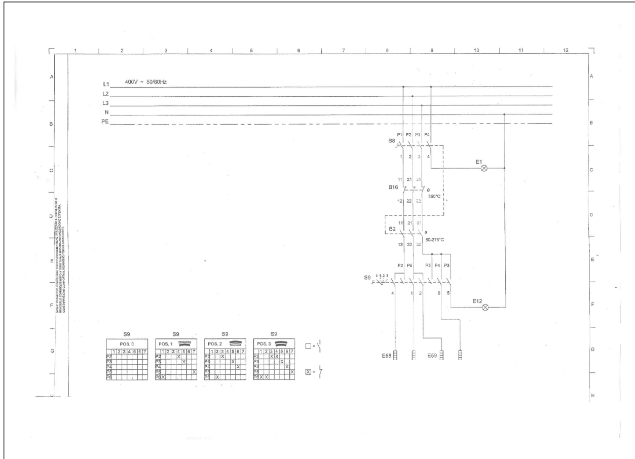
Fig. 26 Wiring diagram 2 - Electric oven
