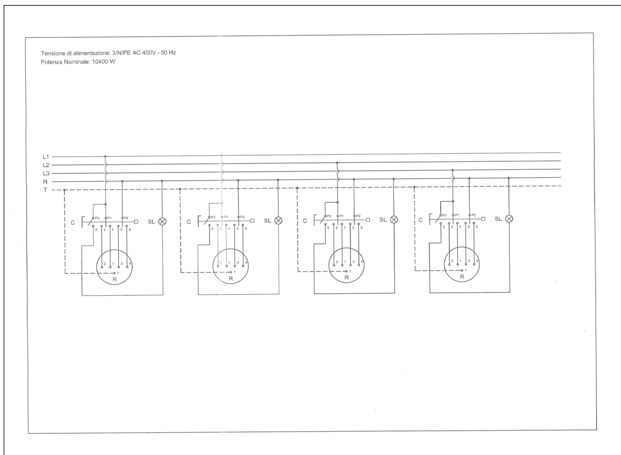
Fig. 25 Wiring diagram 1 - Equipment
