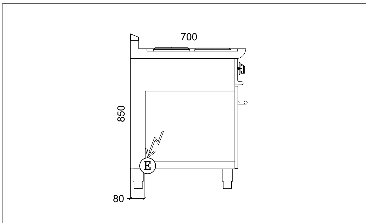
Fig. 17 Range with closed cabinet or oven dimensions
